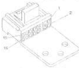
Accessory Connector Block
