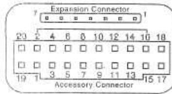
Radio's Accessory Connector
